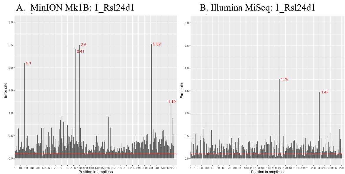
Figure B5 Average error rate (%) at each position along the 1_Rsl24d1 microhaplotype amplicon across caribou samples sequenced with a MinION Mk1B (A) and an Illumina MiSeq (B).
