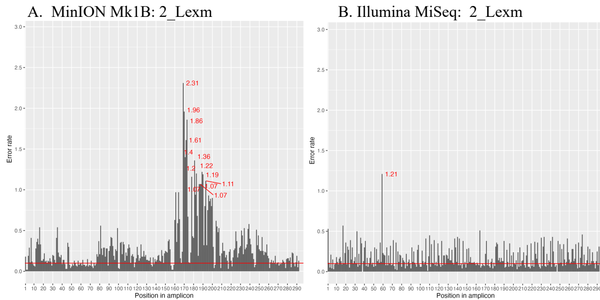
Figure B7 Average error rate (%) at each position along the 2_Lexm microhaplotype amplicon across caribou samples sequenced with a MinION Mk1B (A) and an Illumina MiSeq (B).
