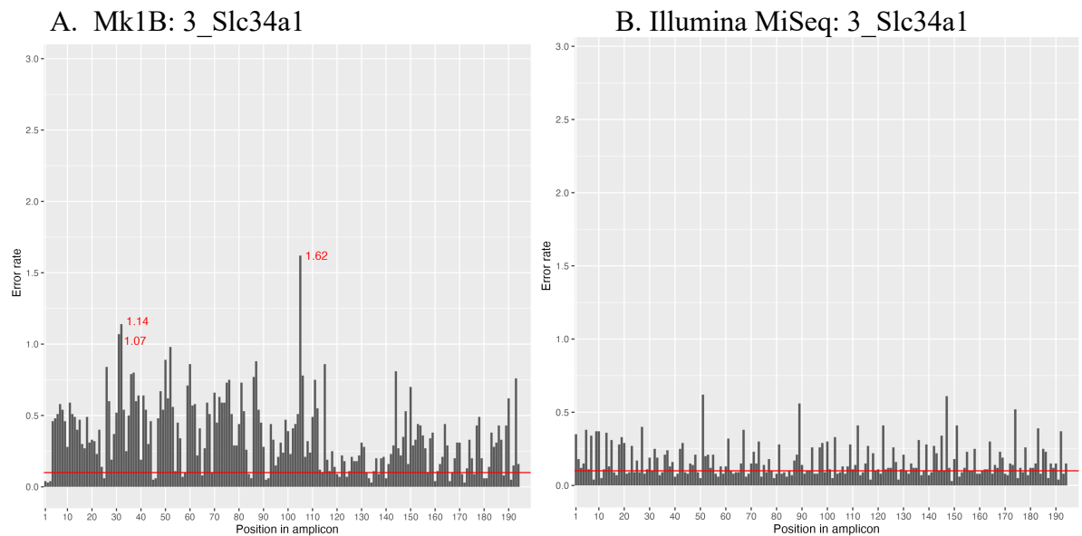
Figure B9 Average error rate (%) at each position along the 3_Slc34a1 microhaplotype amplicon across caribou samples sequenced with a MinION Mk1B (A) and an Illumina MiSeq (B).
