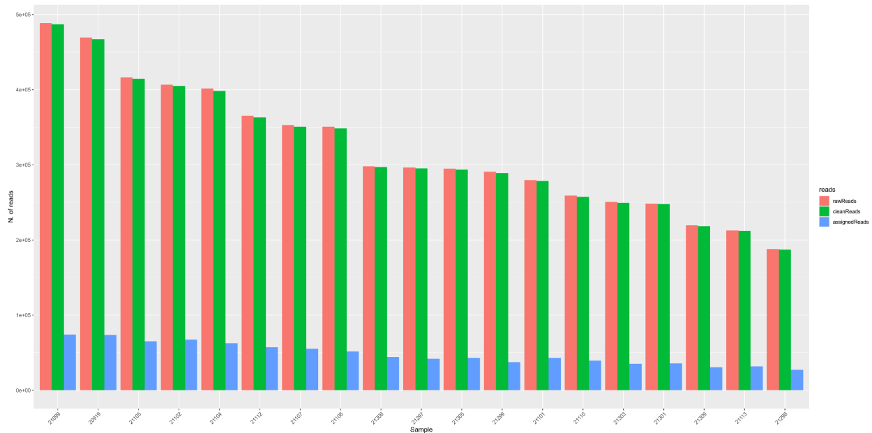
Figure 1.3 Total number of rawReads (raw reads) in red, cleanReads (clean reads) in green, and assignedReads (assigned reads) in blue per caribou sample that passed the quality score threshold generated from microsatellite sequencing on the MinION Mk1B platform. An average of 320,551 raw reads, 318,970 clean reads, and 48,268 assigned reads were obtained per sample.
