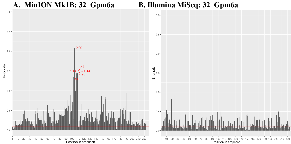
Figure 2.14 Mean error rate (%) at each position along the 32_Gpm6a microhaplotype amplicon across caribou samples sequenced with a MinION Mk1B (A) and an Illumina MiSeq (B).
