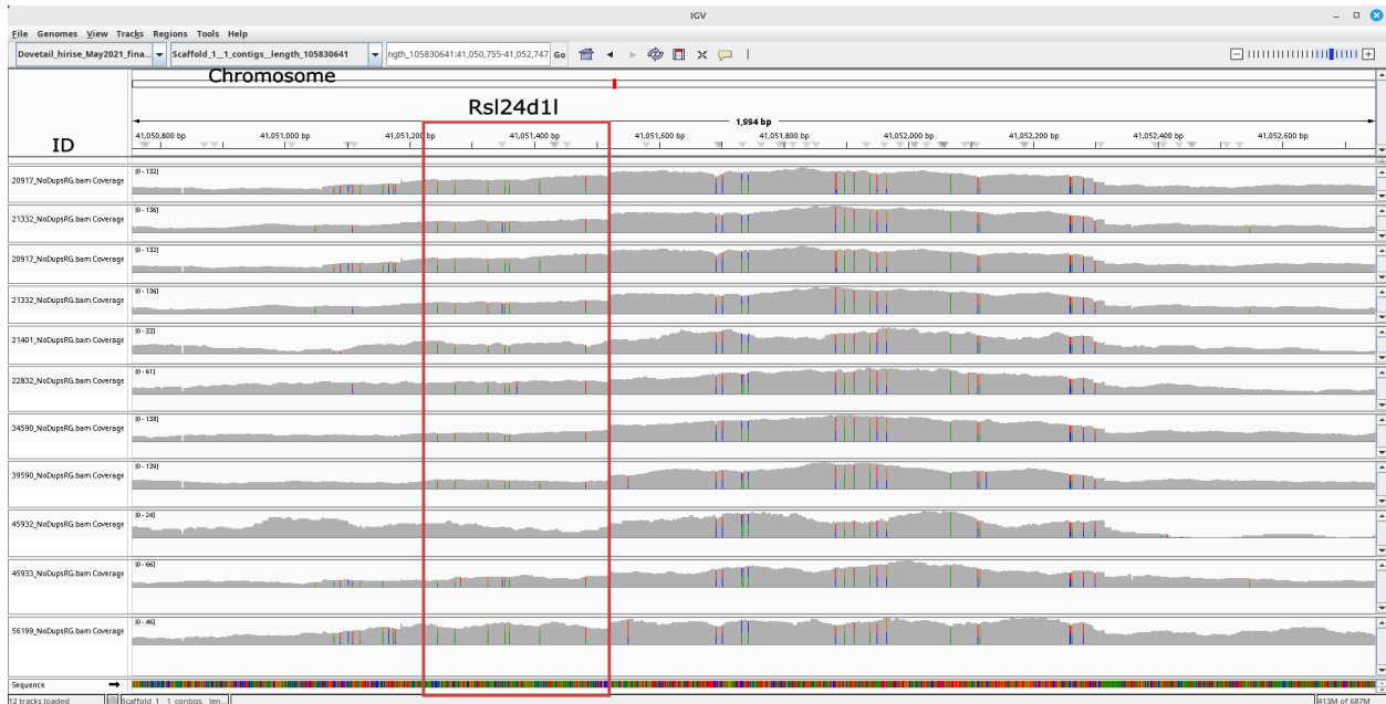
Figure 2.8 Image from Integrated Genomics Viewer (IGV) exemplifying a microhaplotype locus (1_Rsl24d1) on scaffold 1 (chromosome 1) of the caribou genome that is likely a duplicated genomic region. The target locus is outlined in red. Each row represents a unique caribou sample. Data was obtained from whole genome sequencing at approximately 30X depth of coverage.
